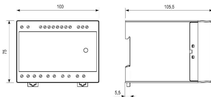
Dimensions for MT440
